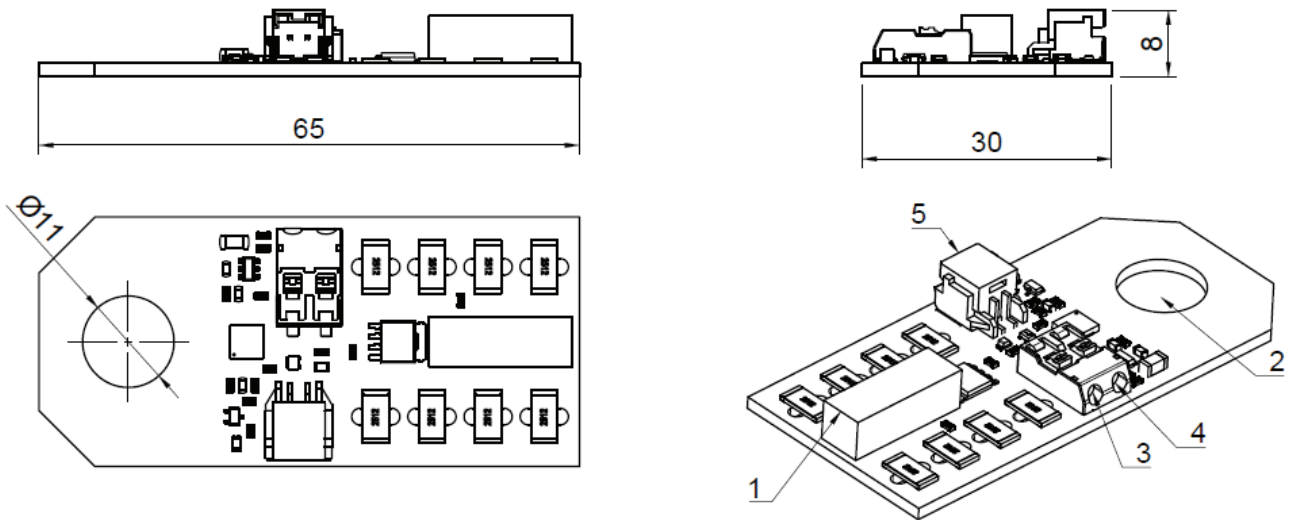
Figure 7.2 EMUS G1 Cell Module 1.5A (CM011A) mechanical drawing. All dimensions in millimeters.
