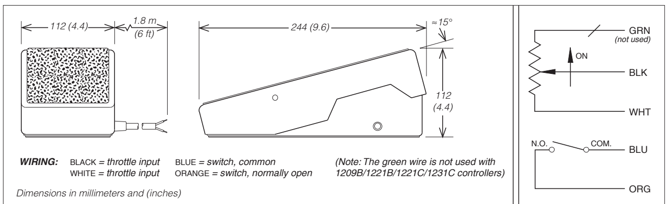
Fig. 5 Curtis PMC footpedal FP-2.
